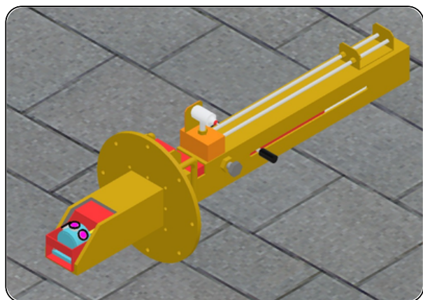
BOTTOM SCAN
